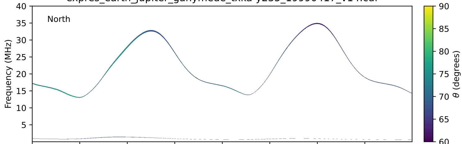
expres_earth_jupiter_ganymede_txka-y235_19990417_v14.cdf
