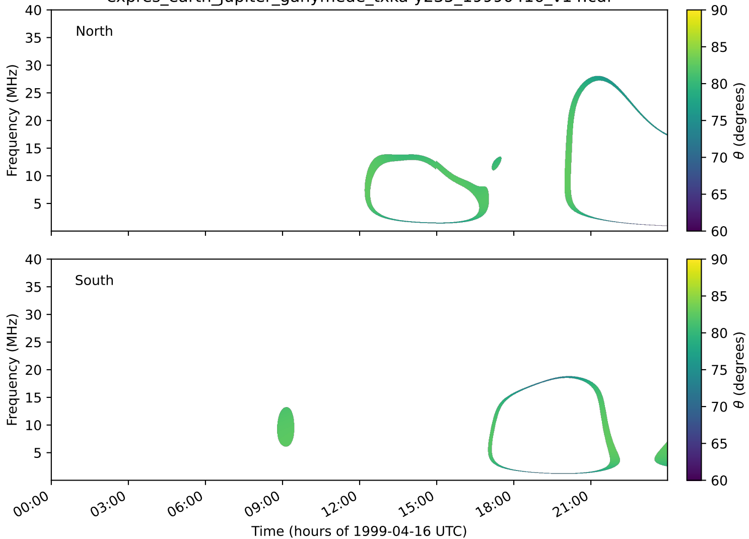
expres_earth_jupiter_ganymede_txka-y235_19990416_v14.cdf
