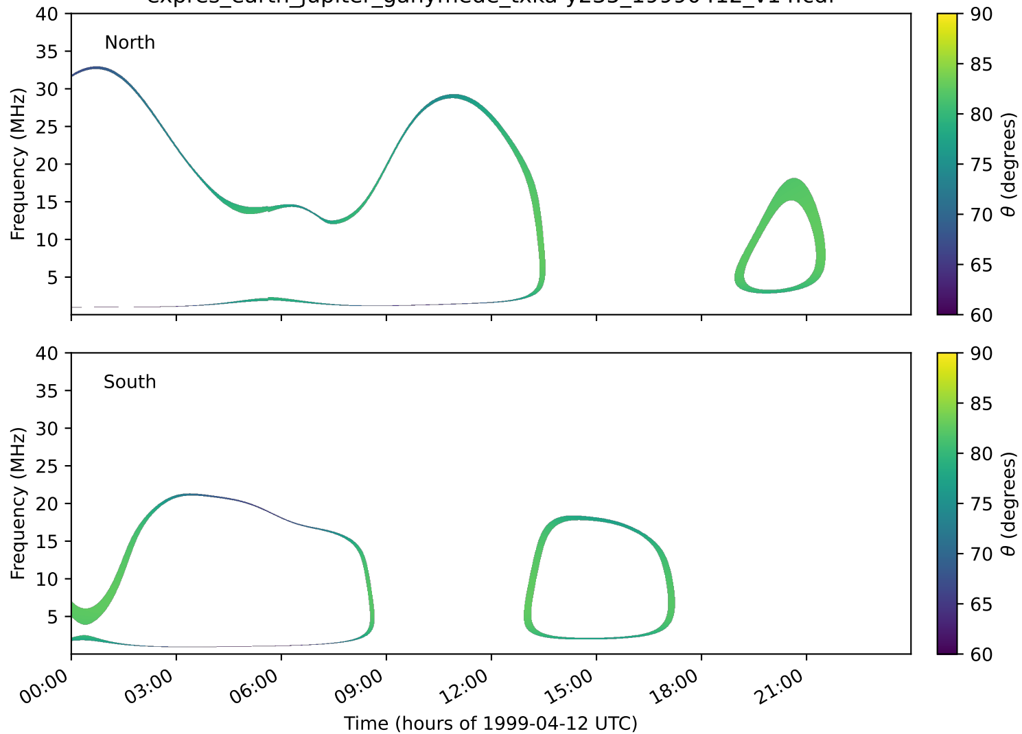
expres_earth_jupiter_ganymede_txka-y235_19990412_v14.cdf
