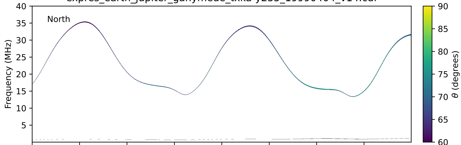
expres_earth_jupiter_ganymede_txka-y235_19990404_v14.cdf
