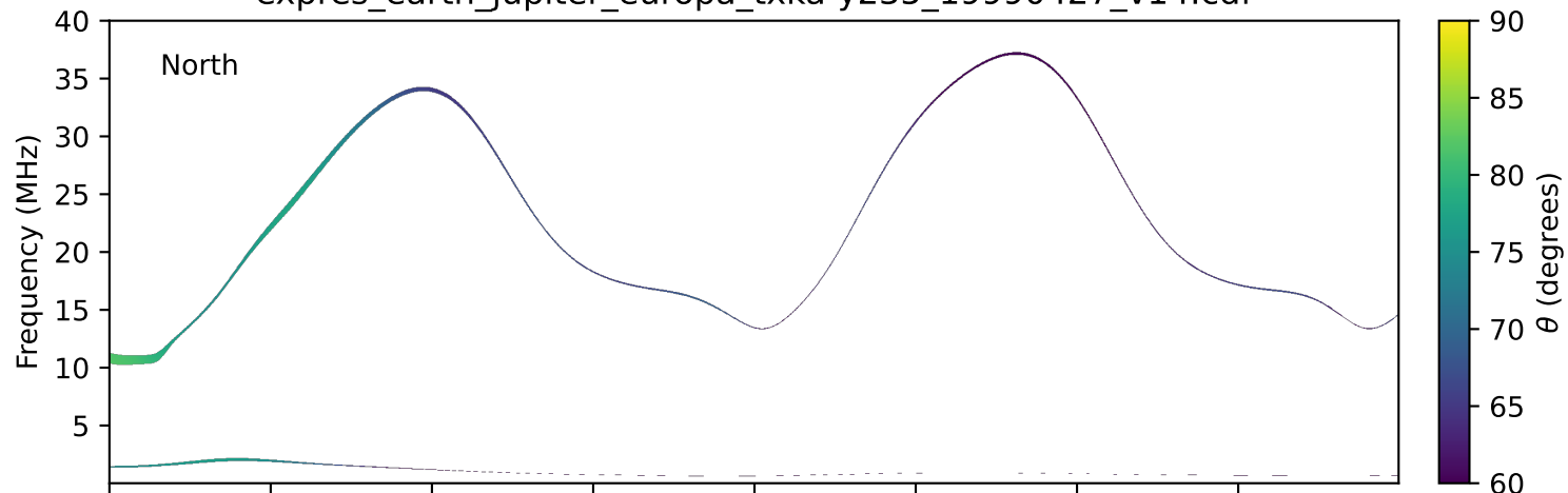
expres_earth_jupiter_europa_txka-y235_19990427_v14.cdf
