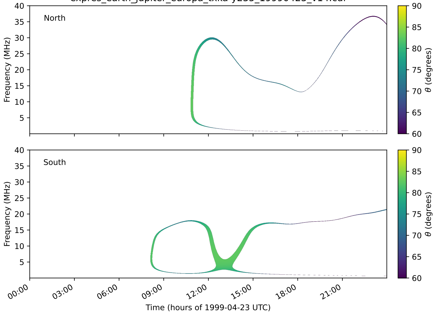
expres_earth_jupiter_europa_txka-y235_19990423_v14.cdf
