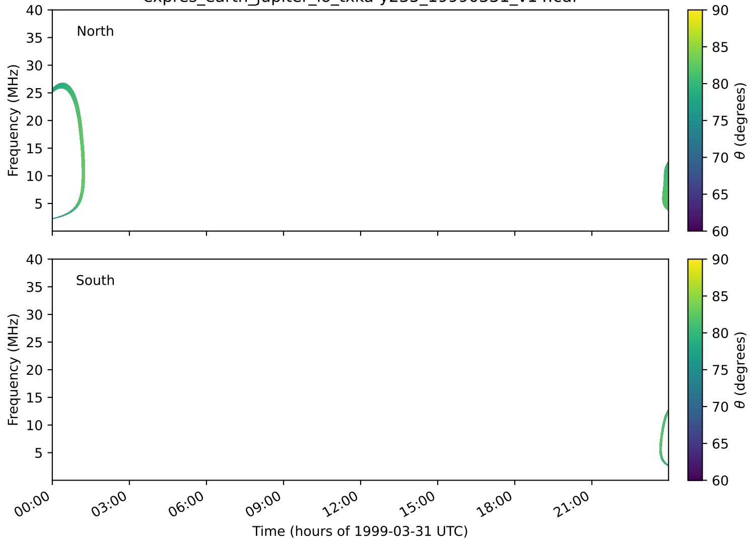
expres_earth_jupiter_io_txka-y235_19990331_v14.cdf
