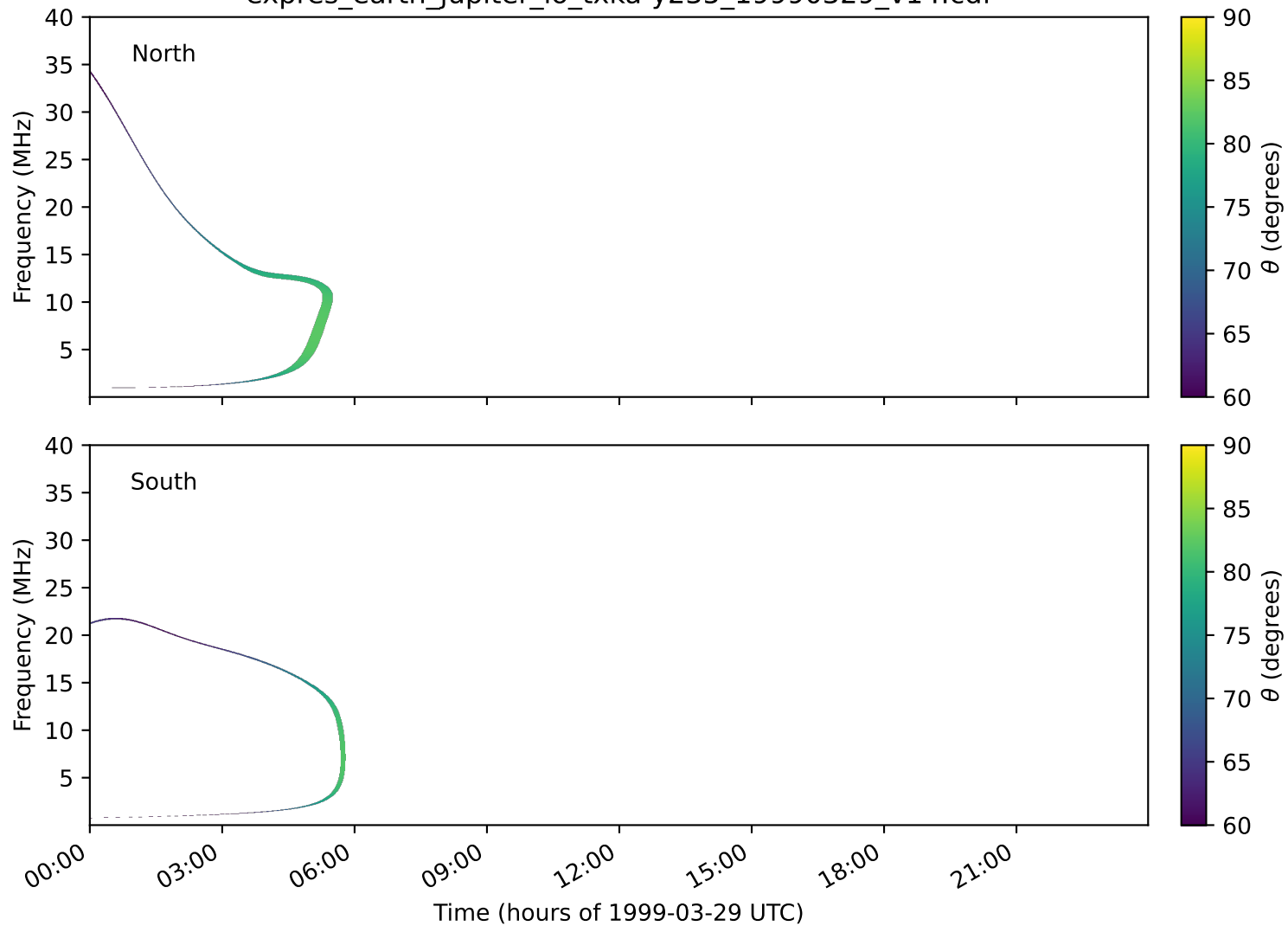
expres_earth_jupiter_io_txka-y235_19990329_v14.cdf
