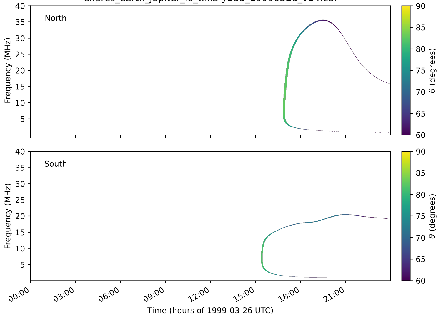
expres_earth_jupiter_io_txka-y235_19990326_v14.cdf
