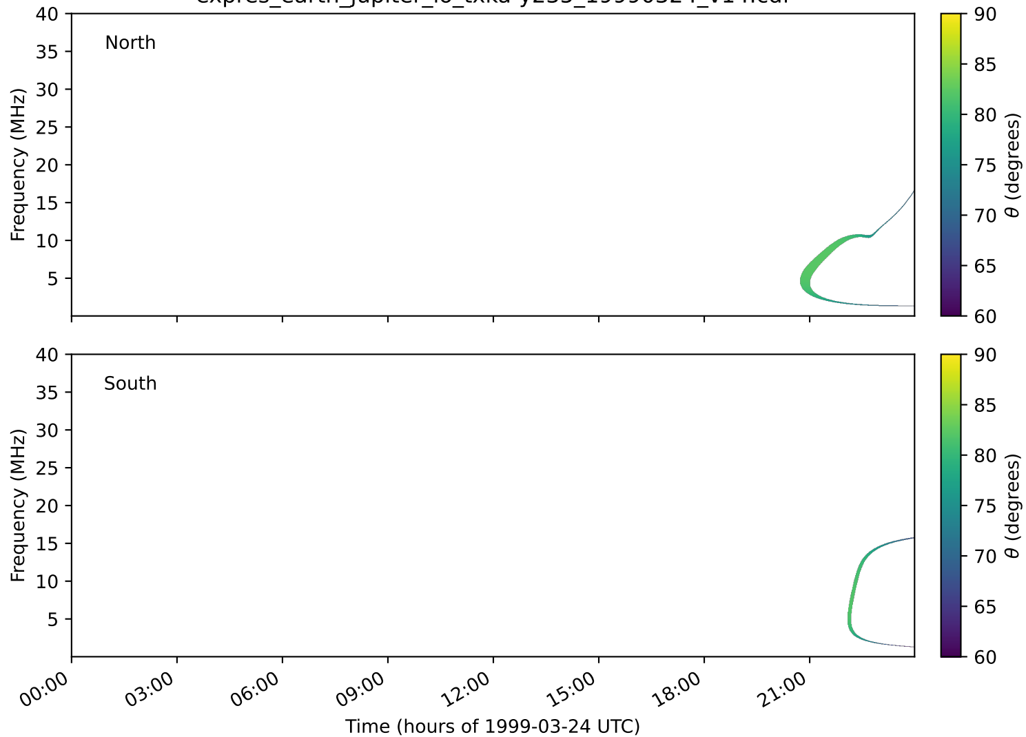
expres_earth_jupiter_io_txka-y235_19990324_v14.cdf
