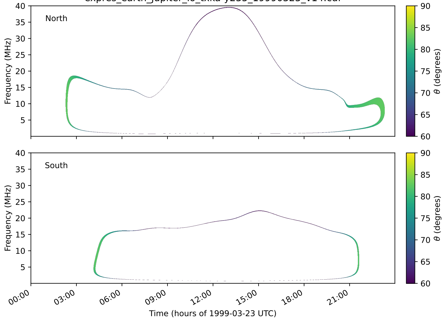
expres_earth_jupiter_io_txka-y235_19990323_v14.cdf
