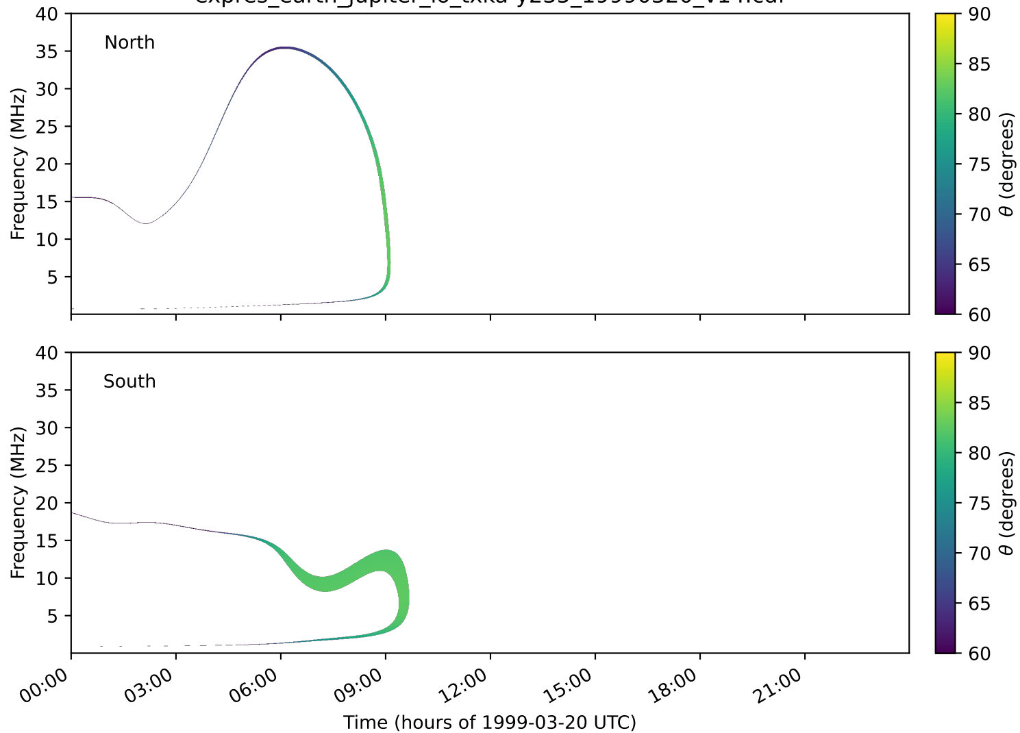
expres_earth_jupiter_io_txka-y235_19990320_v14.cdf
