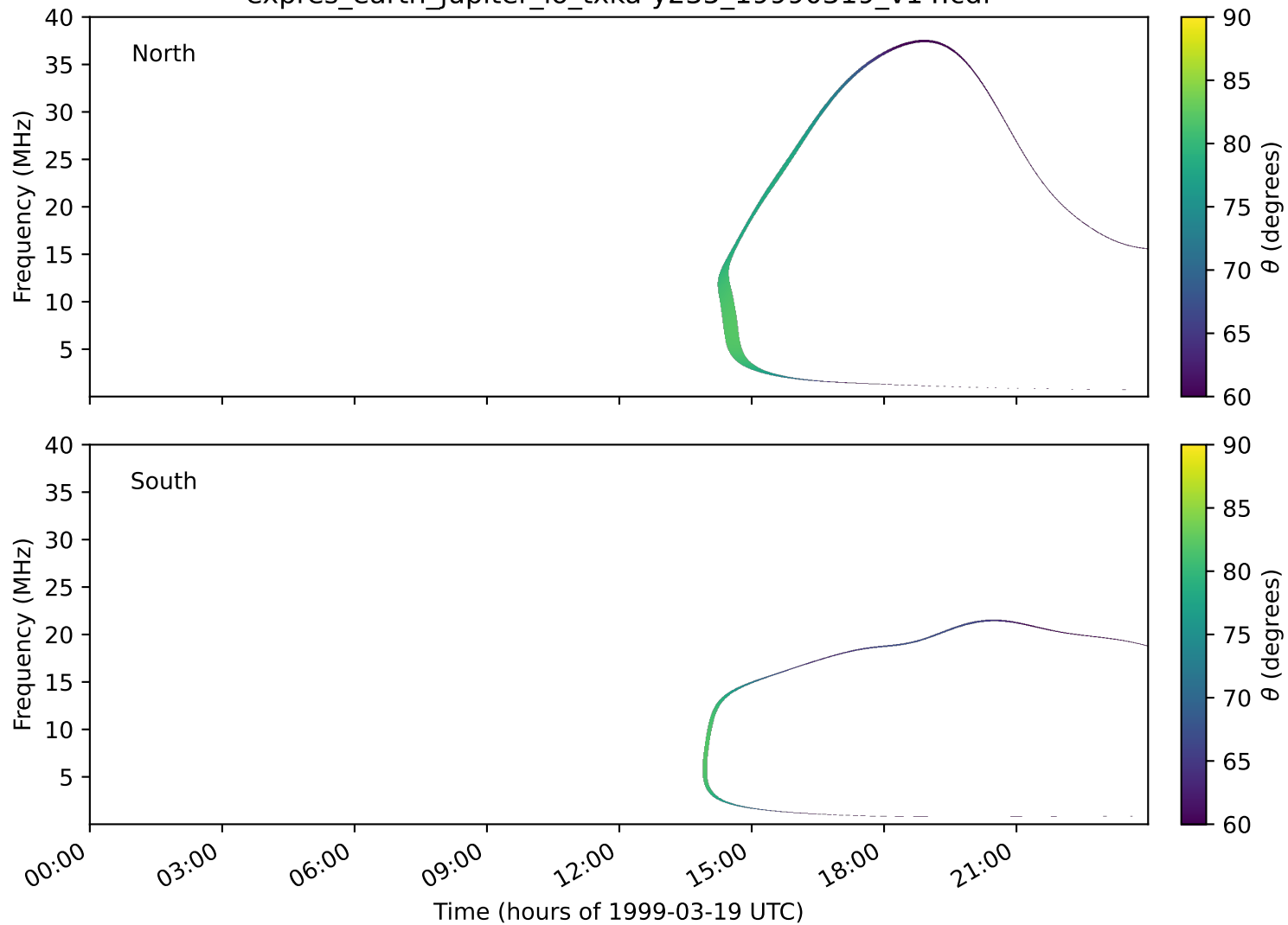
expres_earth_jupiter_io_txka-y235_19990319_v14.cdf
