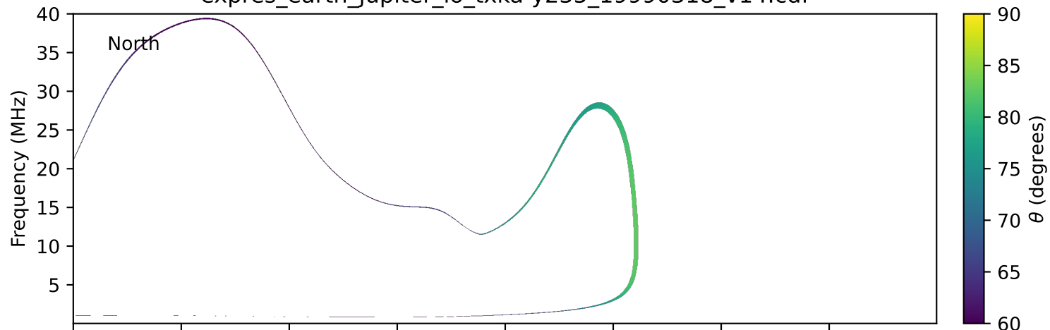
expres_earth_jupiter_io_txka-y235_19990318_v14.cdf
