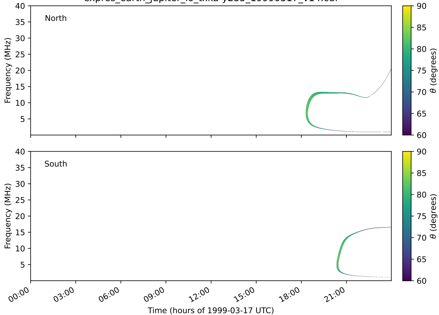
expres_earth_jupiter_io_txka-y235_19990317_v14.cdf
