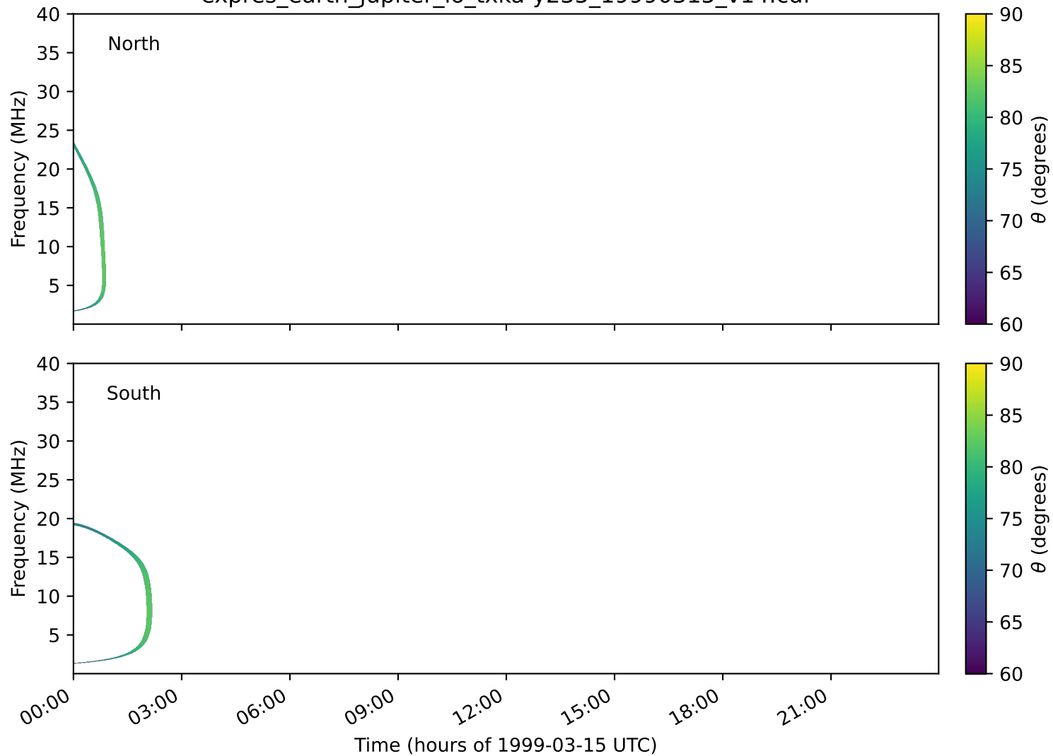
expres_earth_jupiter_io_txka-y235_19990315_v14.cdf
