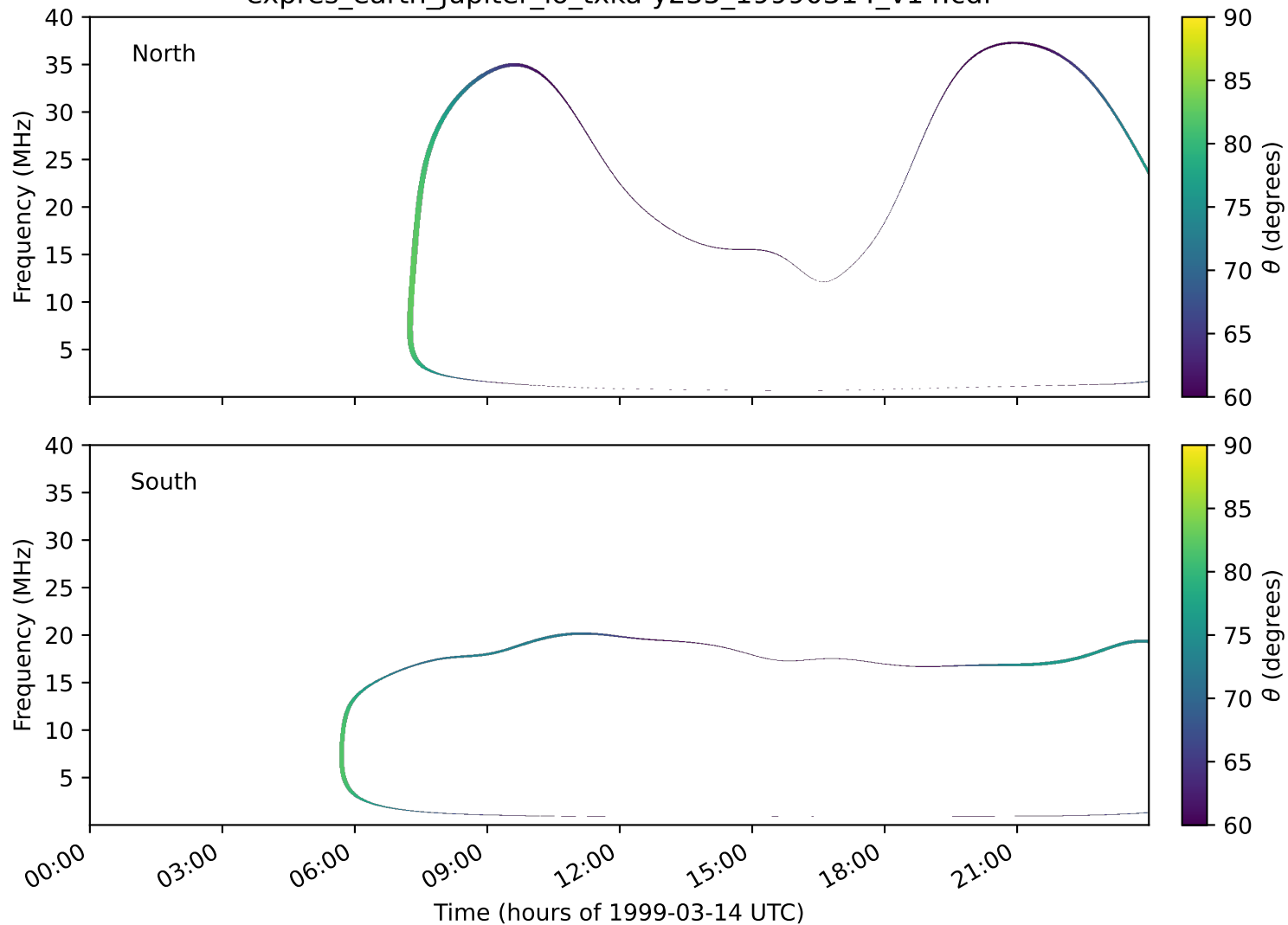
expres_earth_jupiter_io_txka-y235_19990314_v14.cdf
