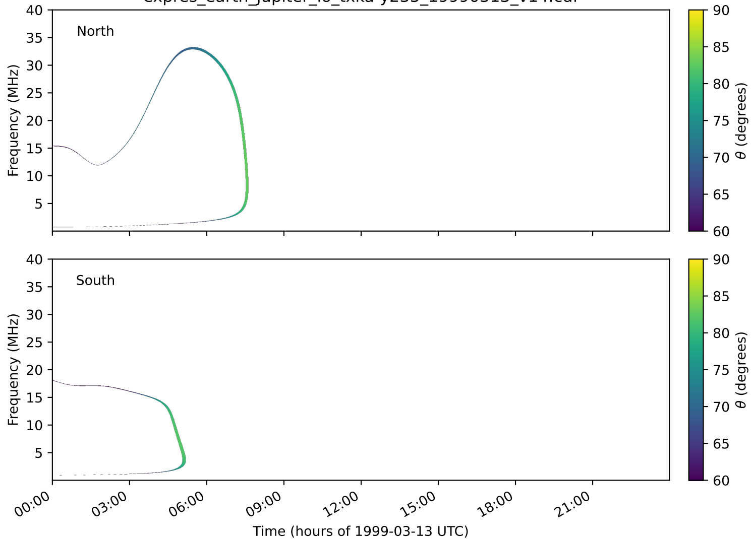
expres_earth_jupiter_io_txka-y235_19990313_v14.cdf
