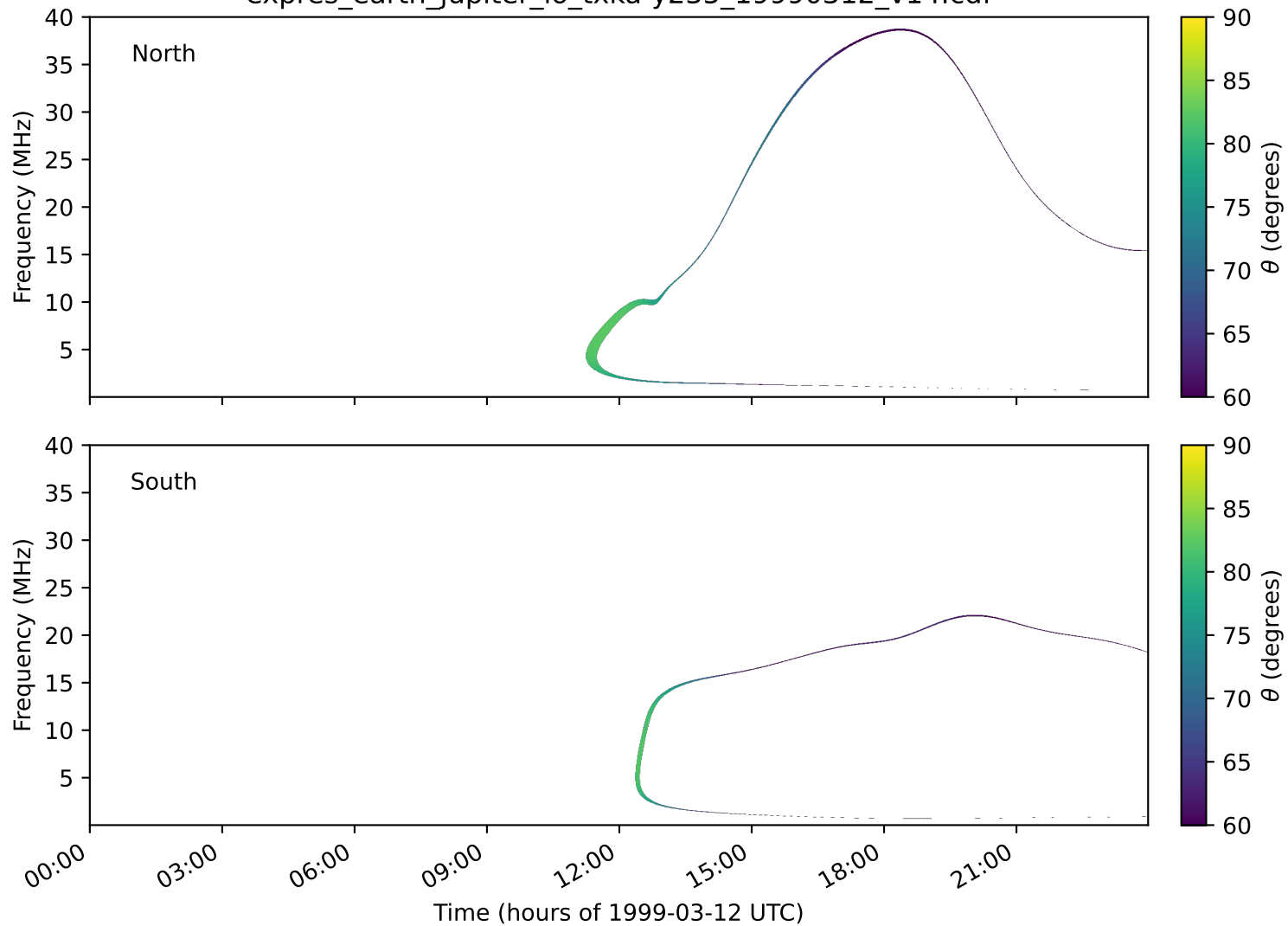
expres_earth_jupiter_io_txka-y235_19990312_v14.cdf
