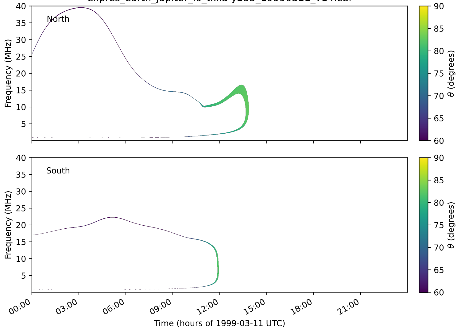
expres_earth_jupiter_io_txka-y235_19990311_v14.cdf
