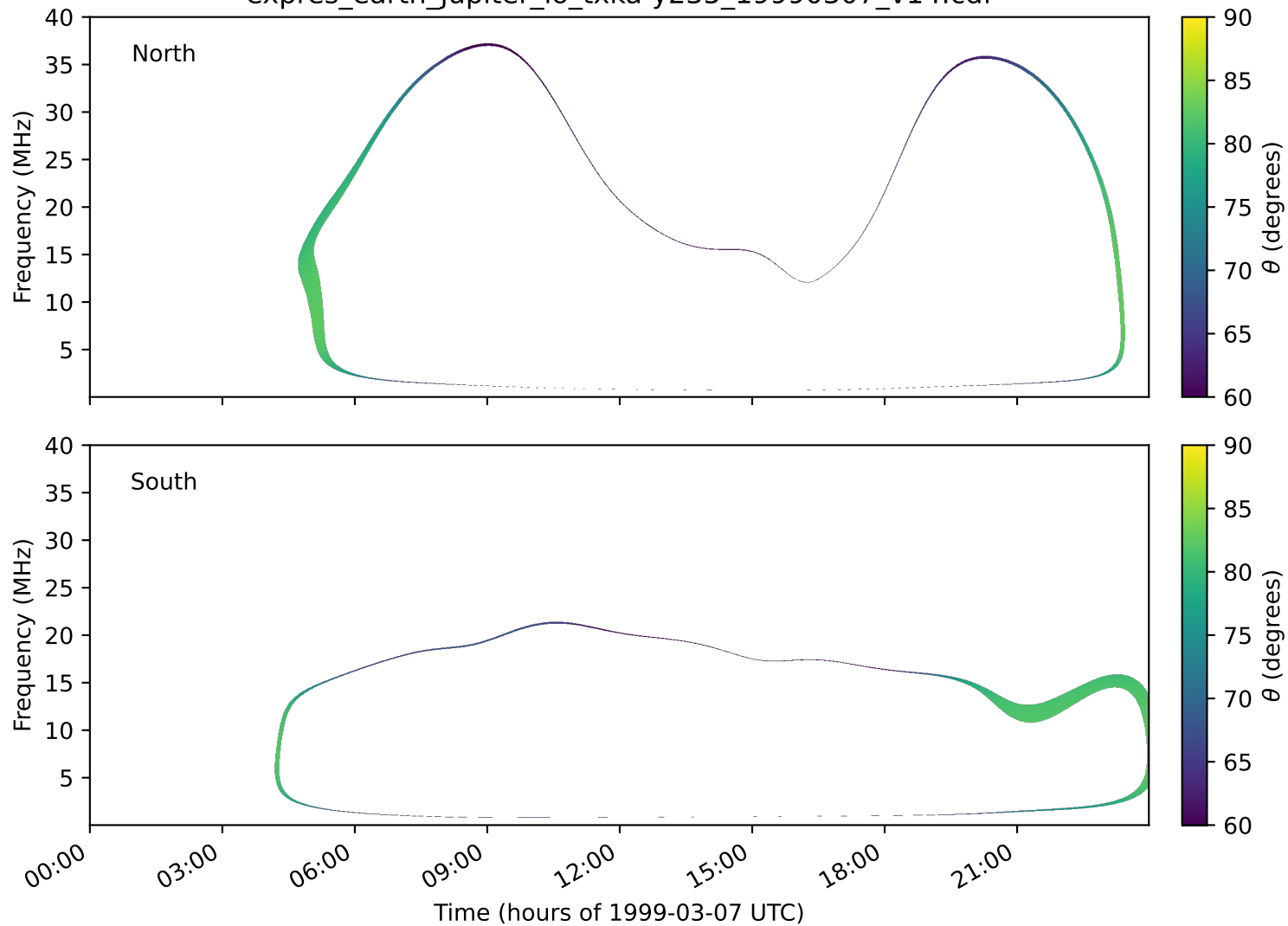
expres_earth_jupiter_io_txka-y235_19990307_v14.cdf
