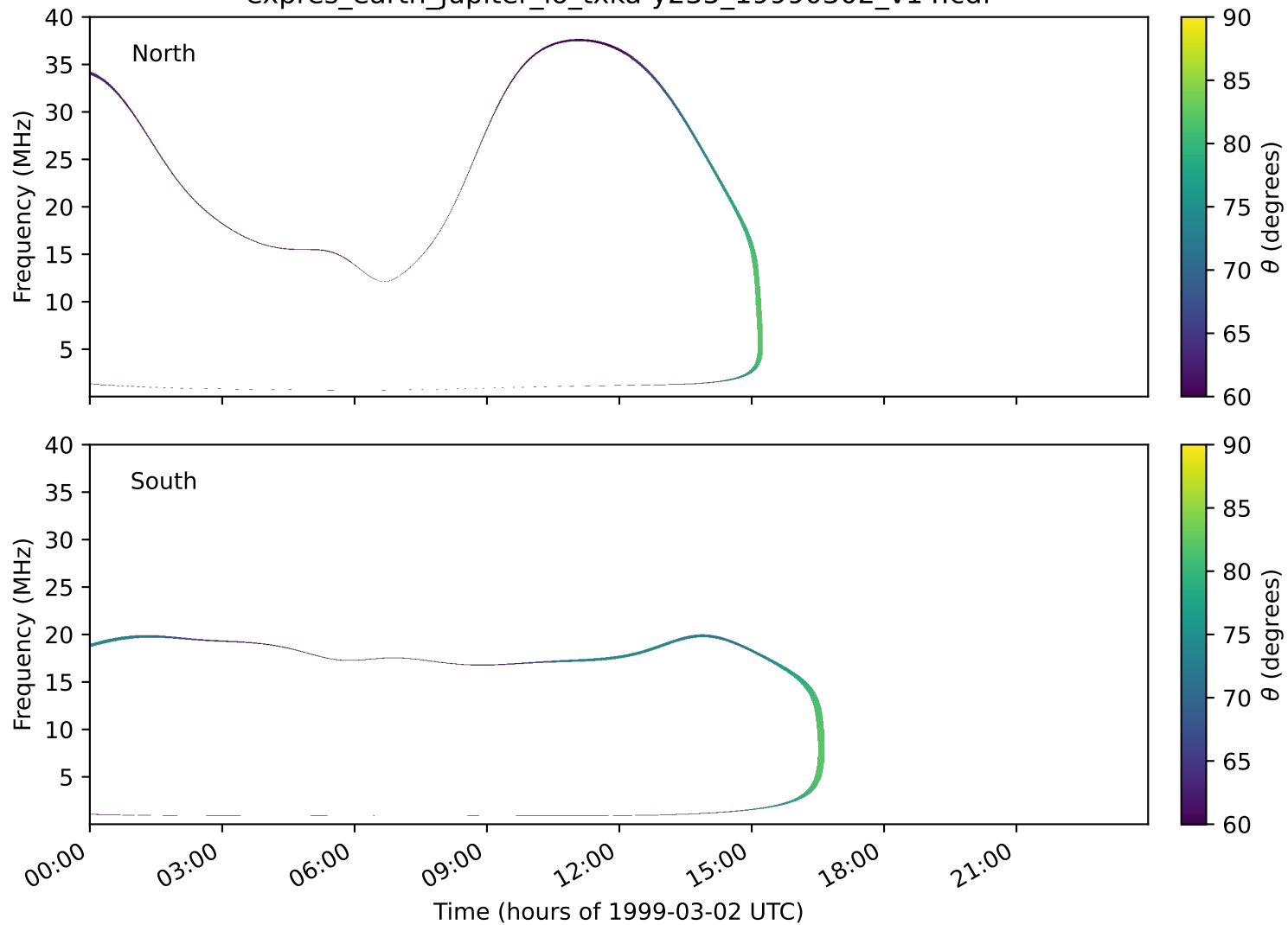
expres_earth_jupiter_io_txka-y235_19990302_v14.cdf
