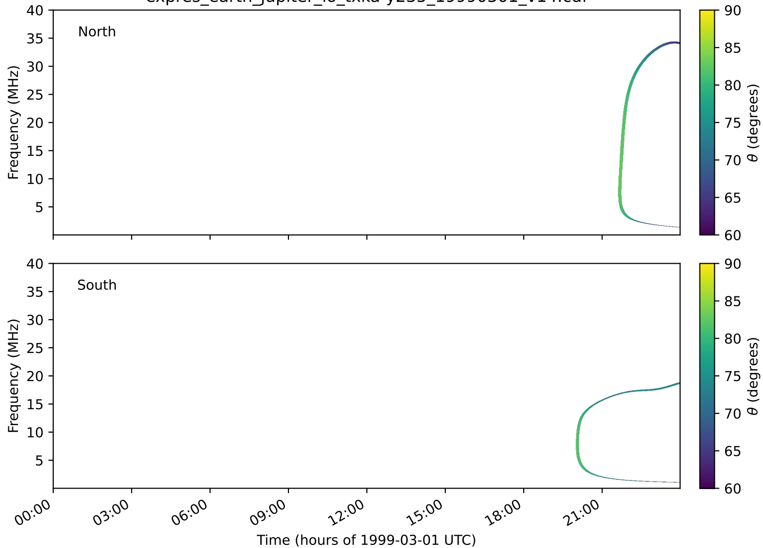
expres_earth_jupiter_io_txka-y235_19990301_v14.cdf
