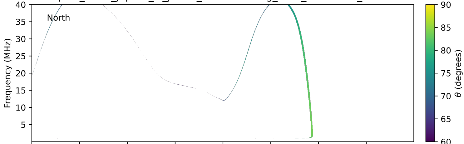
expres_earth_jupiter_io_jrm09_lossc-wid1deg_3kev_19990325_v11.cdf
