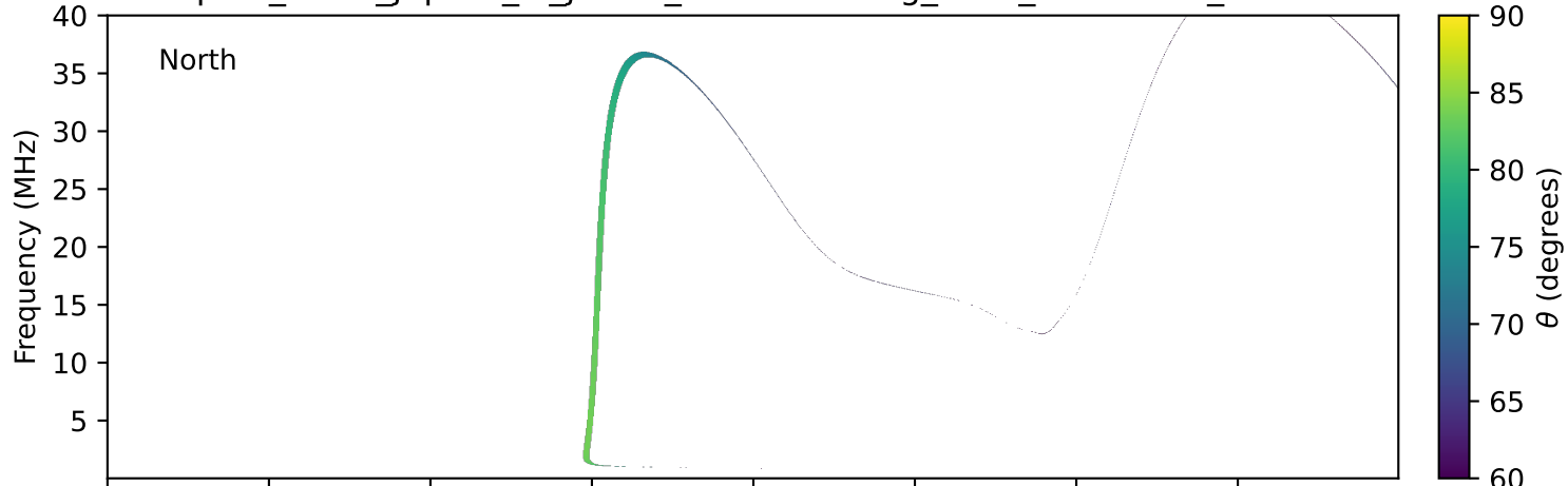
expres_earth_jupiter_io_jrm09_lossc-wid1deg_3kev_19990321_v11.cdf
