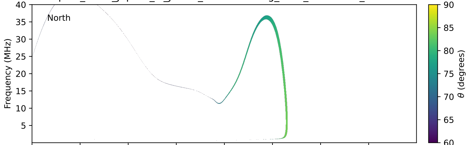
expres_earth_jupiter_io_jrm09_lossc-wid1deg_3kev_19990318_v11.cdf
