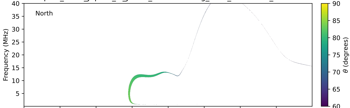
expres_earth_jupiter_io_jrm09_lossc-wid1deg_3kev_19990305_v11.cdf
