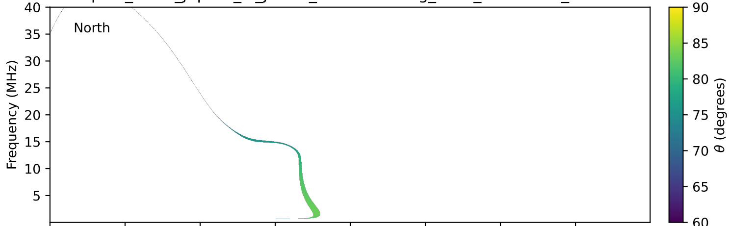
expres_earth_jupiter_io_jrm09_lossc-wid1deg_3kev_19990304_v11.cdf
