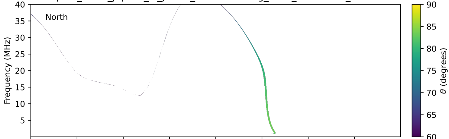
expres_earth_jupiter_io_jrm09_lossc-wid1deg_3kev_19990302_v11.cdf
