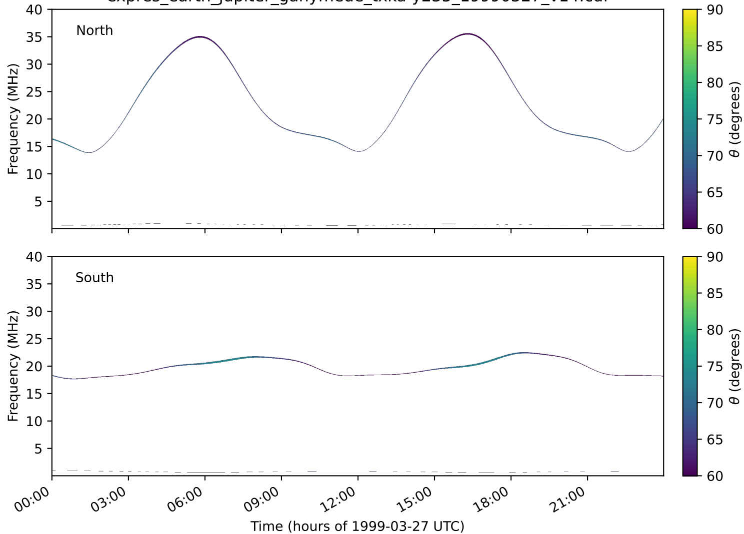
expres_earth_jupiter_ganymede_txka-y235_19990327_v14.cdf
