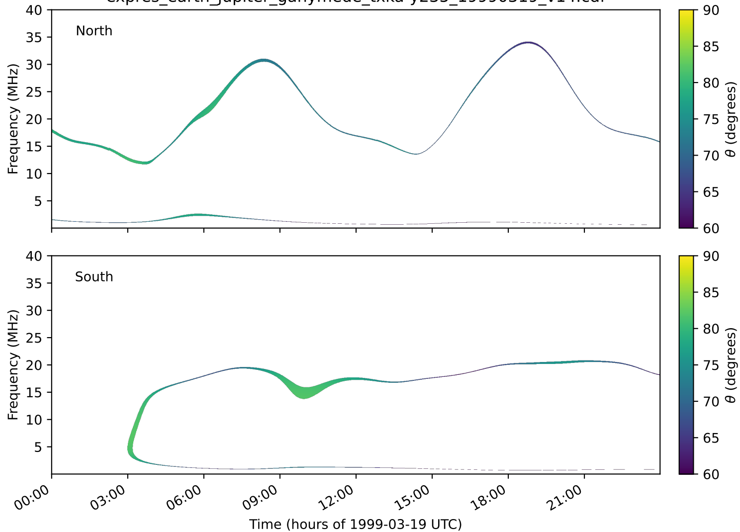
expres_earth_jupiter_ganymede_txka-y235_19990319_v14.cdf
