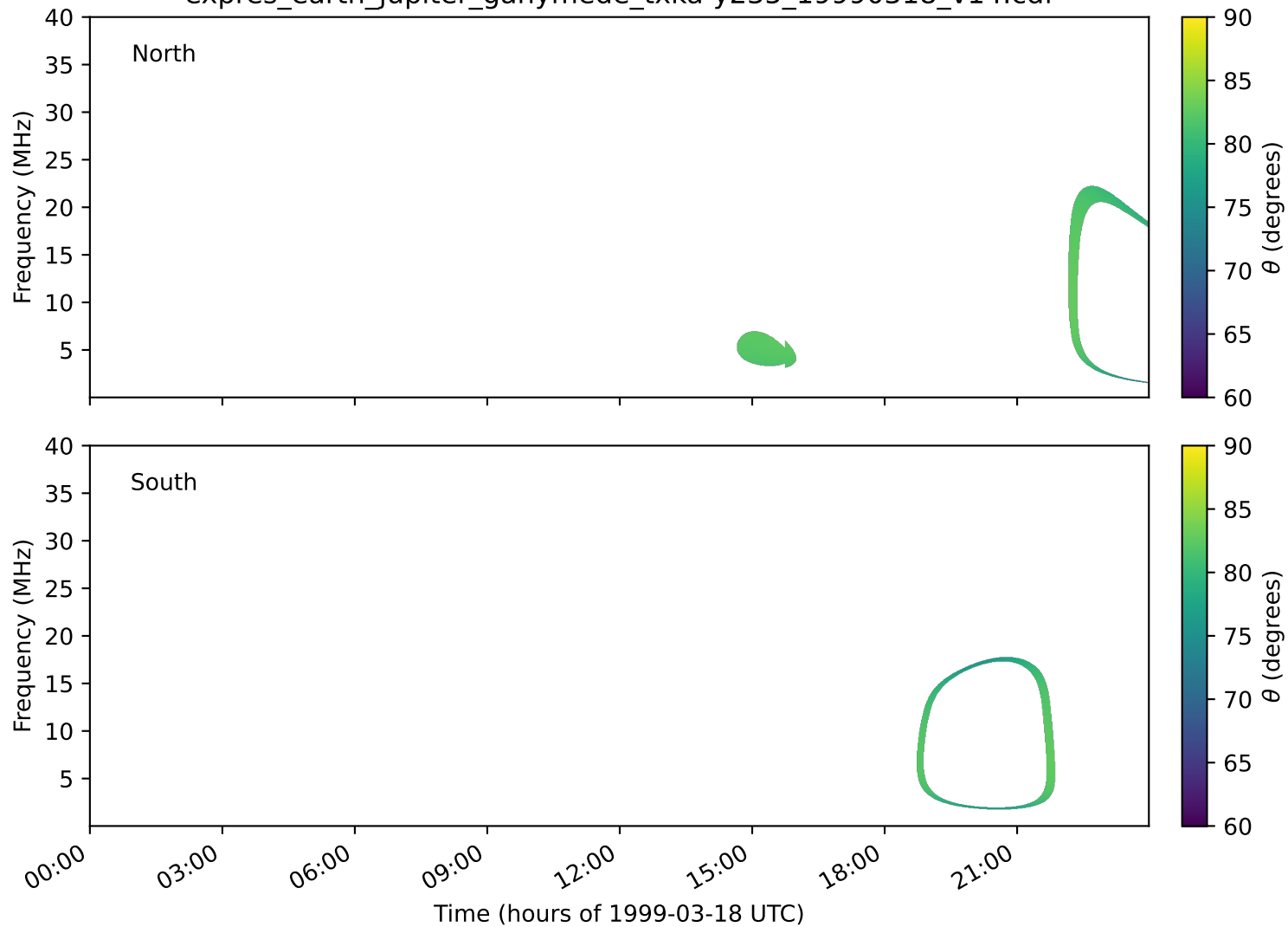
expres_earth_jupiter_ganymede_txka-y235_19990318_v14.cdf
