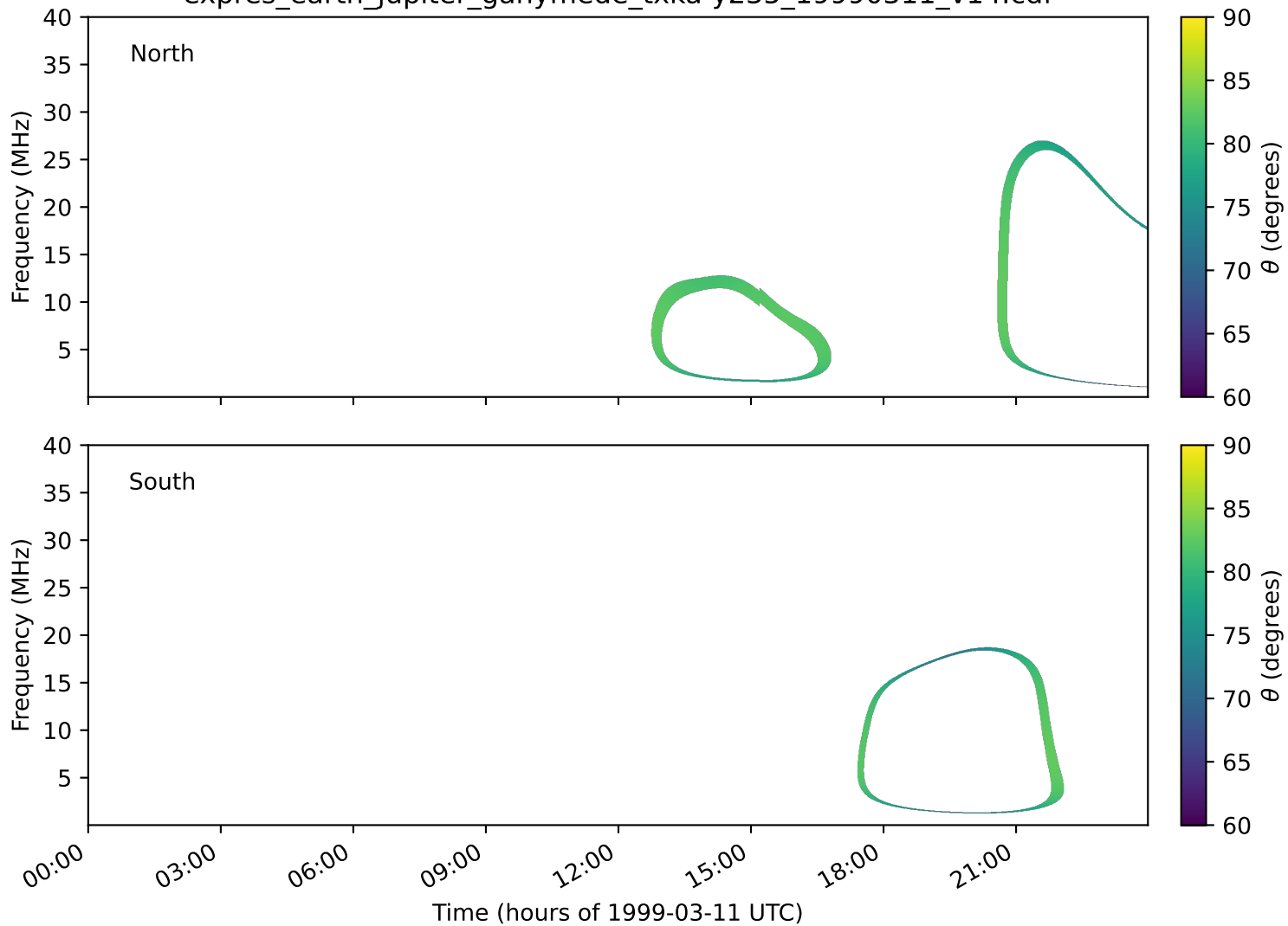
expres_earth_jupiter_ganymede_txka-y235_19990311_v14.cdf
