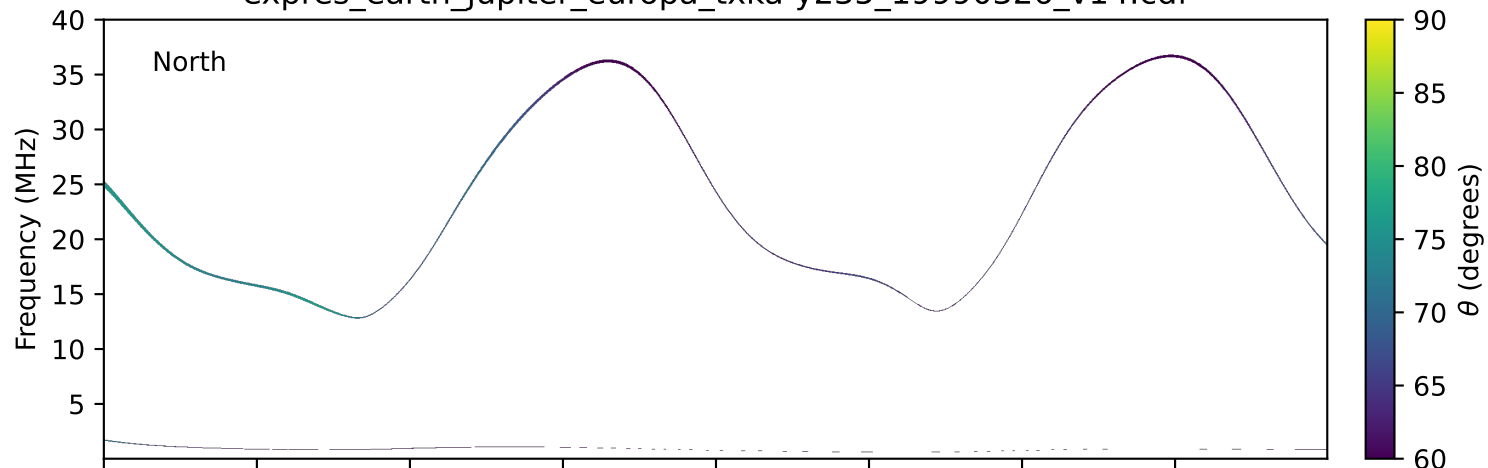
expres_earth_jupiter_europa_txka-y235_19990326_v14.cdf
