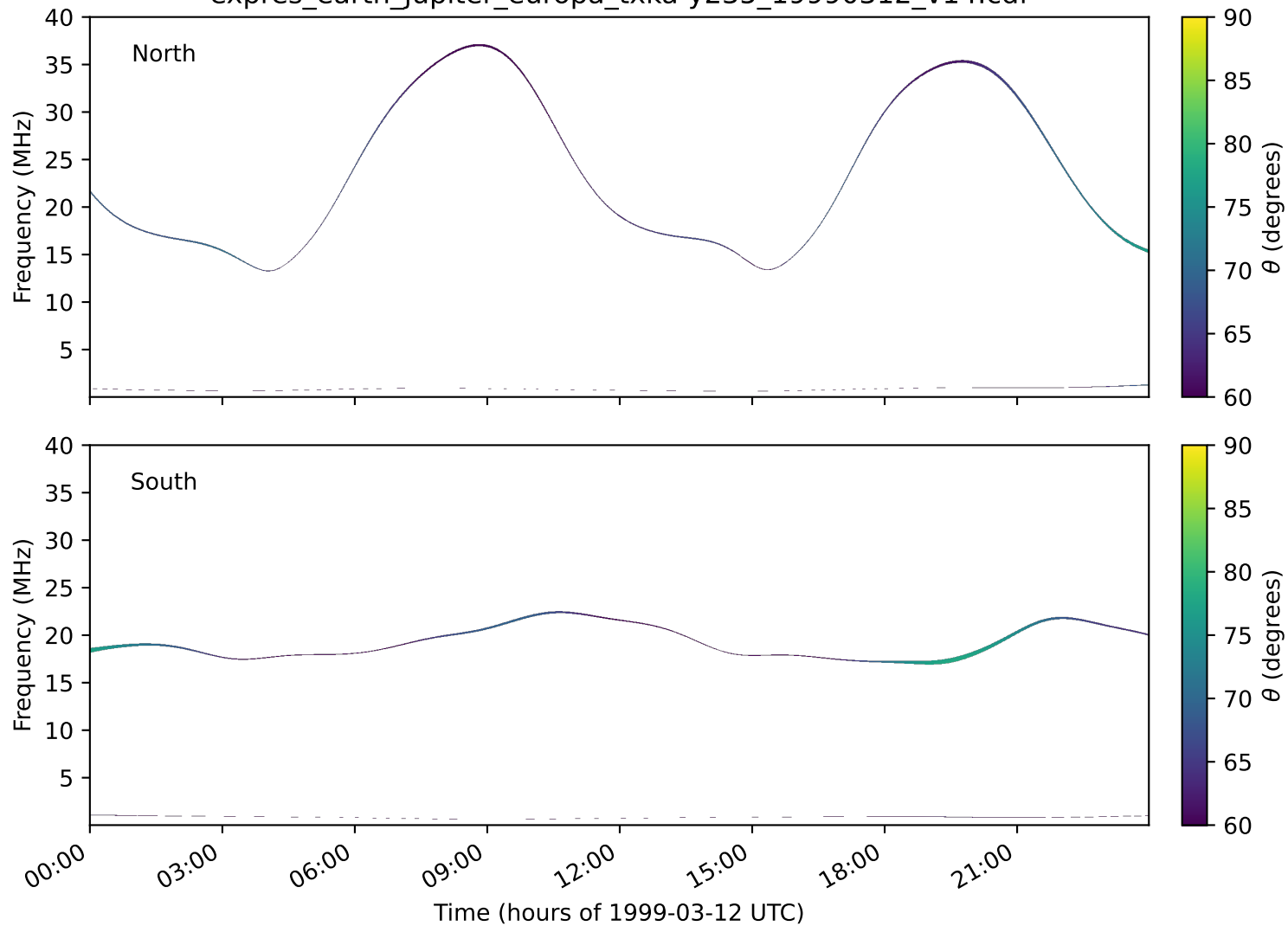
expres_earth_jupiter_europa_txka-y235_19990312_v14.cdf
