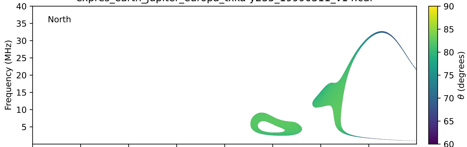
expres_earth_jupiter_europa_txka-y235_19990311_v14.cdf
