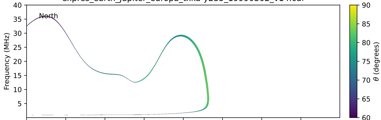
expres_earth_jupiter_europa_txka-y235_19990302_v14.cdf
