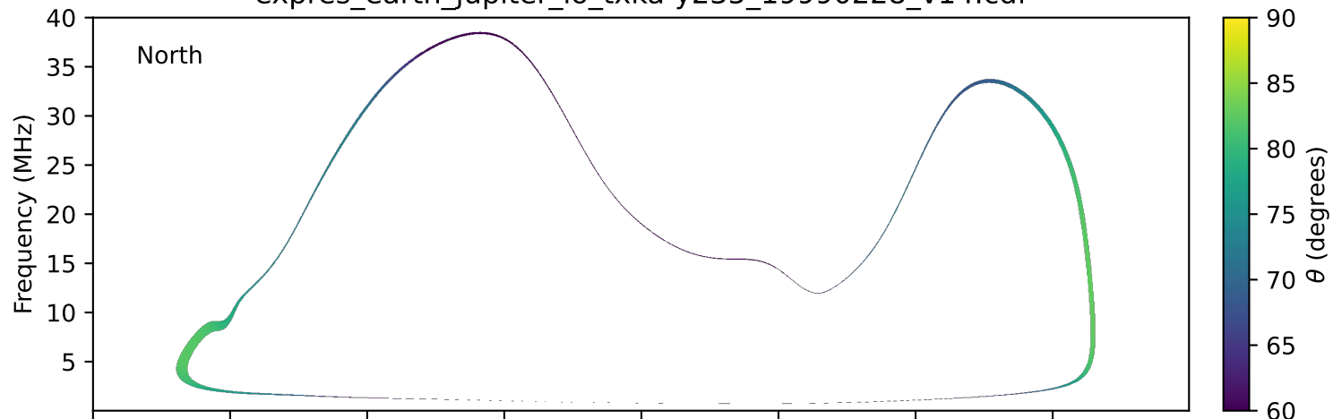
expres_earth_jupiter_io_txka-y235_19990228_v14.cdf
