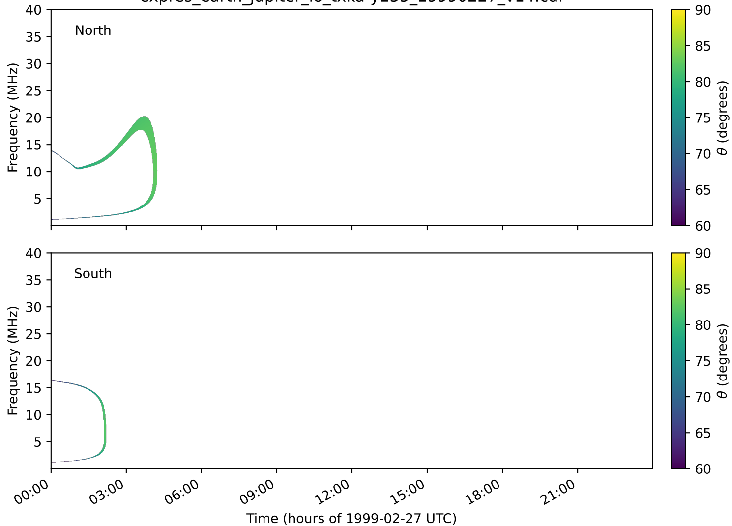
expres_earth_jupiter_io_txka-y235_19990227_v14.cdf
