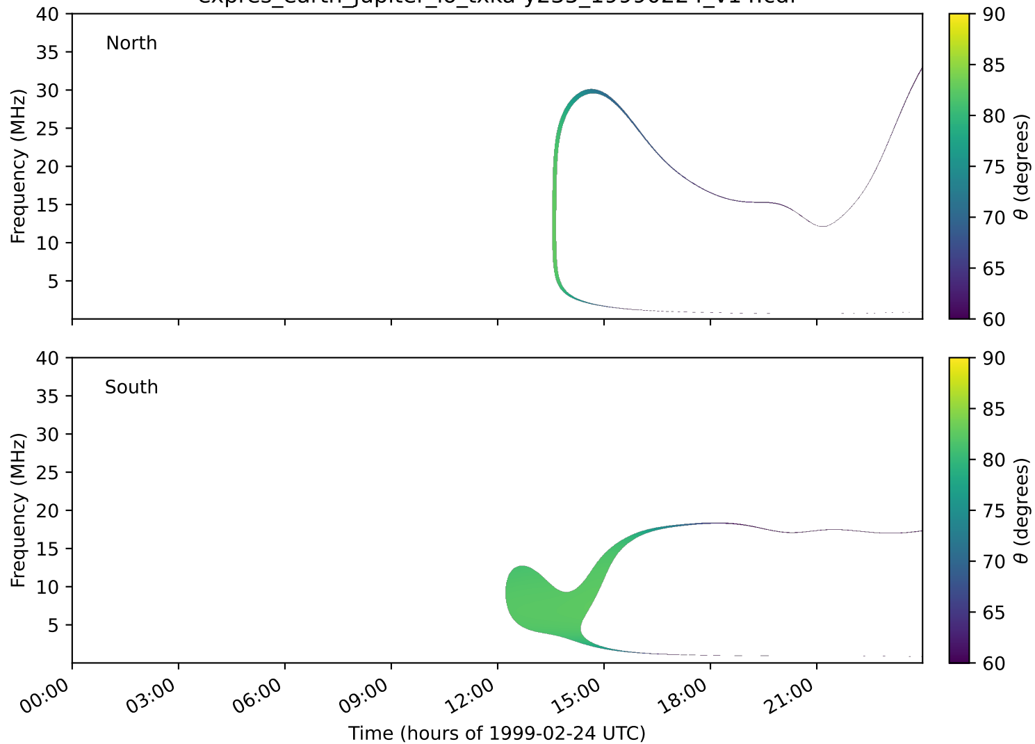
expres_earth_jupiter_io_txka-y235_19990224_v14.cdf
