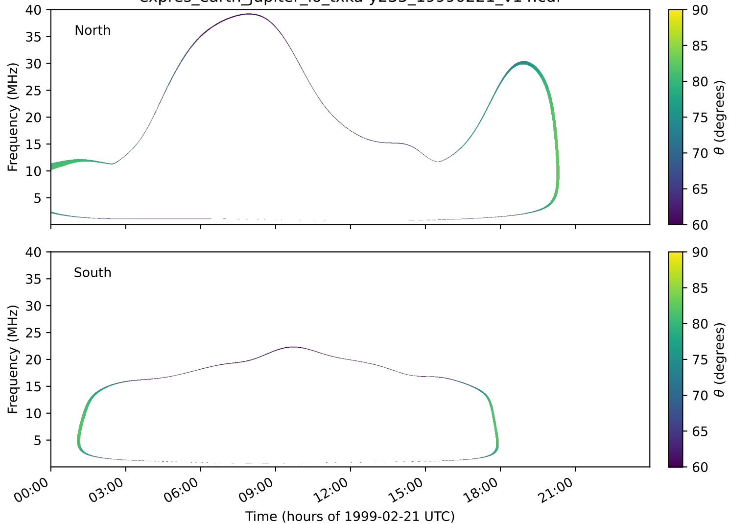
expres_earth_jupiter_io_txka-y235_19990221_v14.cdf
