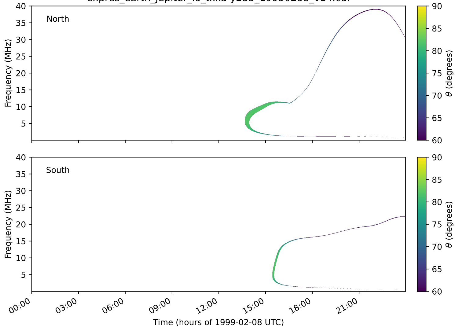
expres_earth_jupiter_io_txka-y235_19990208_v14.cdf
