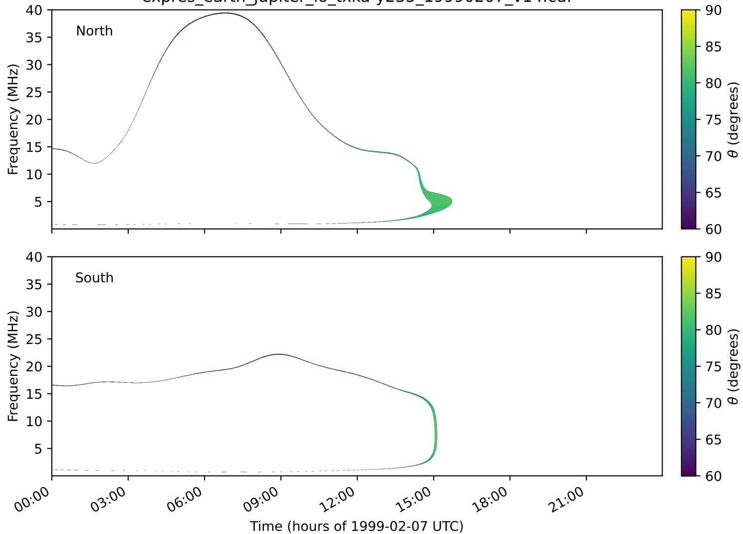
expres_earth_jupiter_io_txka-y235_19990207_v14.cdf
