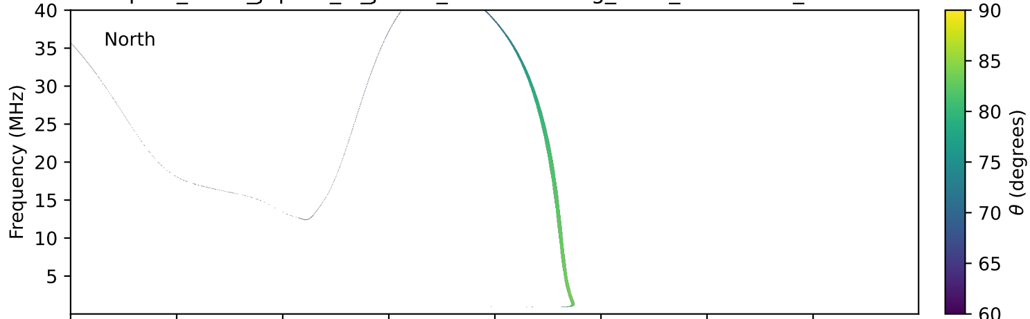
expres_earth_jupiter_io_jrm09_lossc-wid1deg_3kev_19990223_v11.cdf
