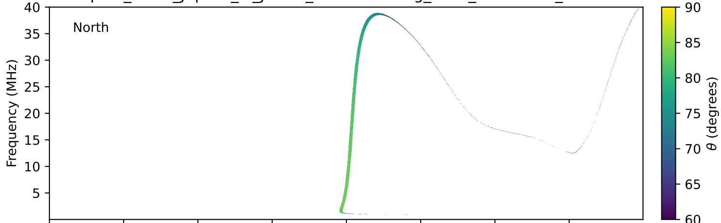
expres_earth_jupiter_io_jrm09_lossc-wid1deg_3kev_19990217_v11.cdf
