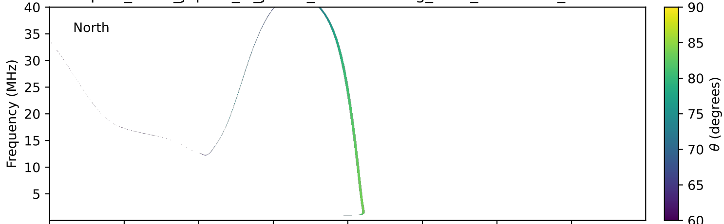
expres_earth_jupiter_io_jrm09_lossc-wid1deg_3kev_19990216_v11.cdf
