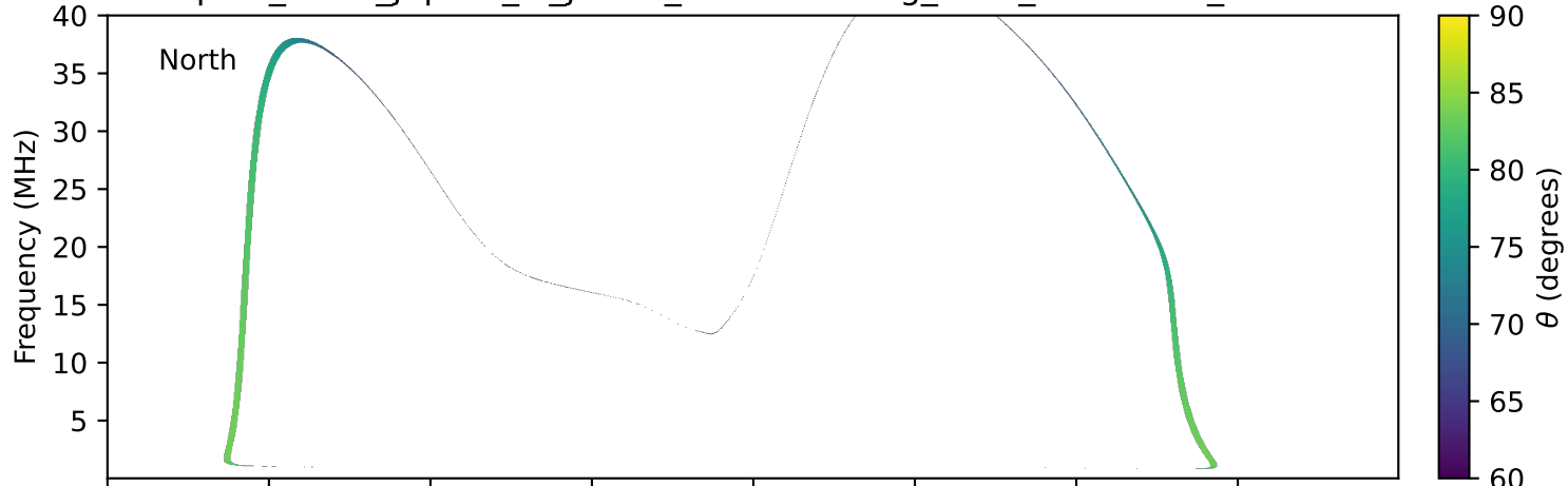
expres_earth_jupiter_io_jrm09_lossc-wid1deg_3kev_19990205_v11.cdf
