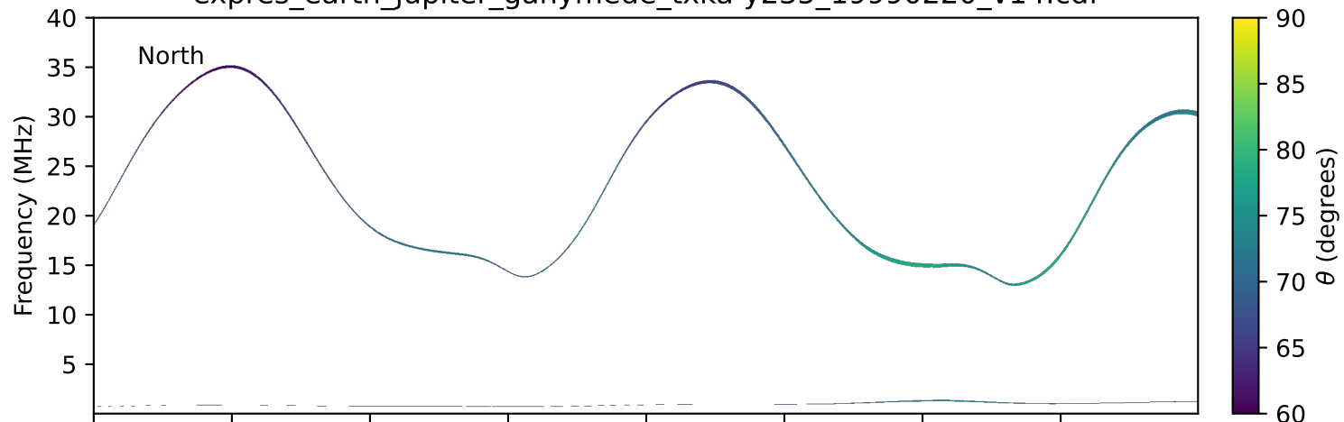
expres_earth_jupiter_ganymede_txka-y235_19990220_v14.cdf
