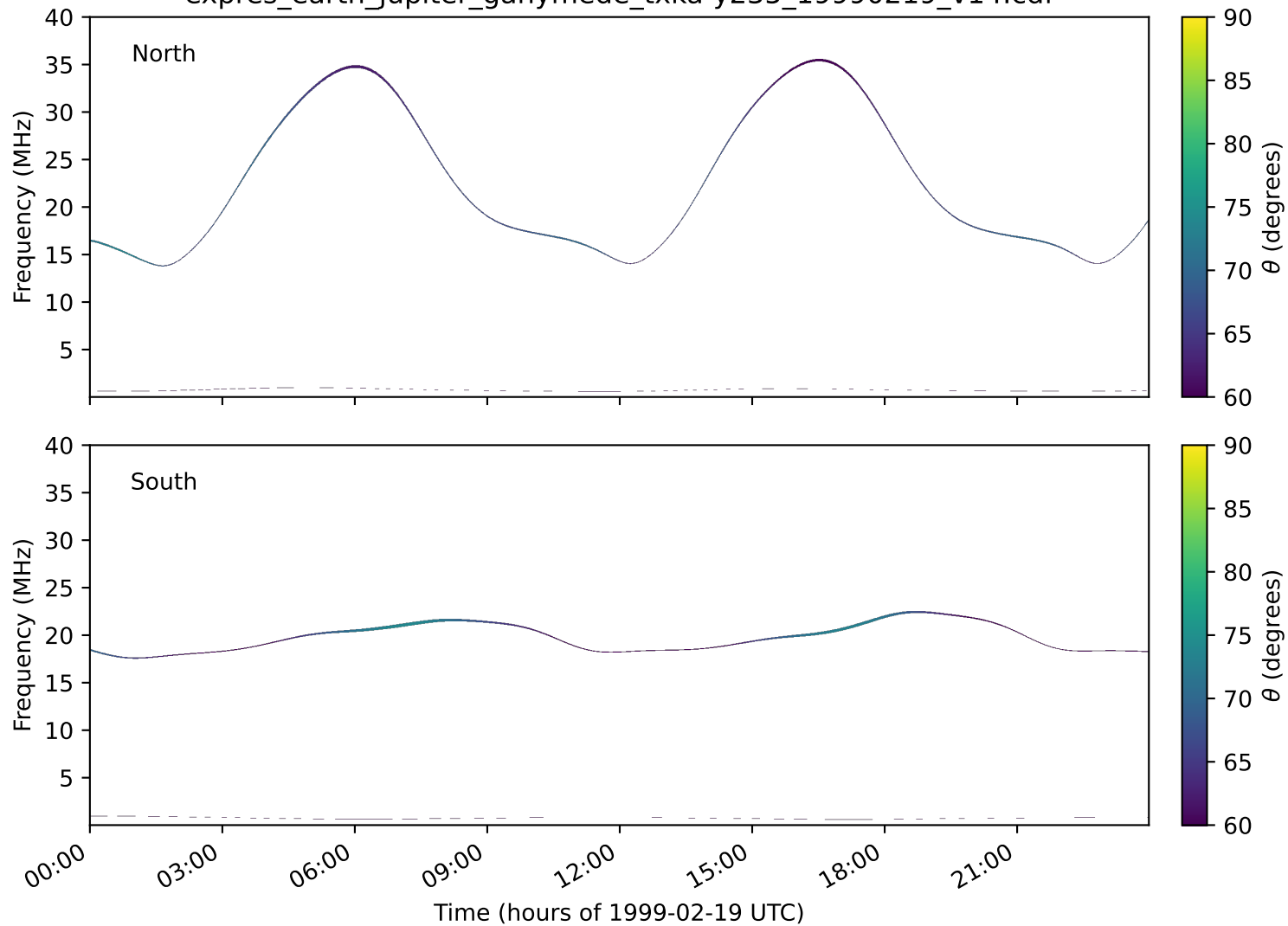
expres_earth_jupiter_ganymede_txka-y235_19990219_v14.cdf
