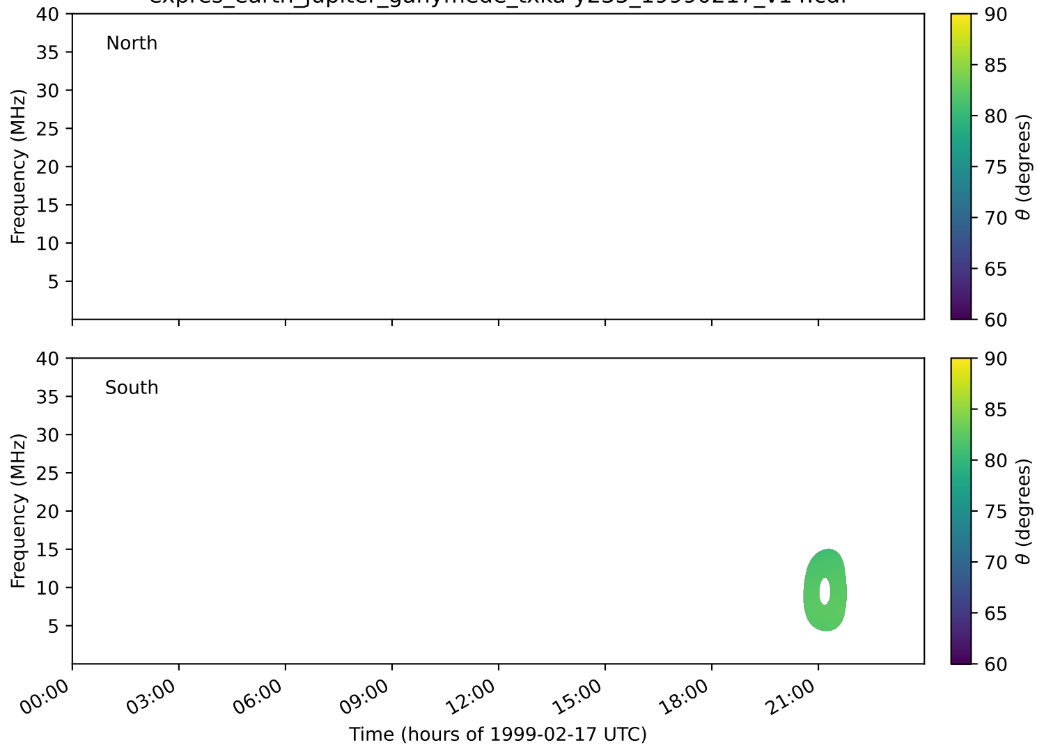
expres_earth_jupiter_ganymede_txka-y235_19990217_v14.cdf
